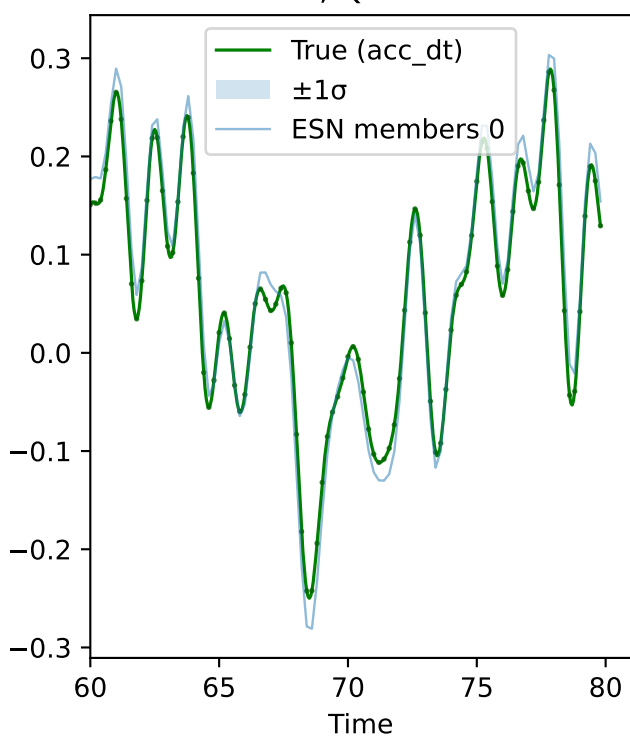
N=5, Qubit=2
