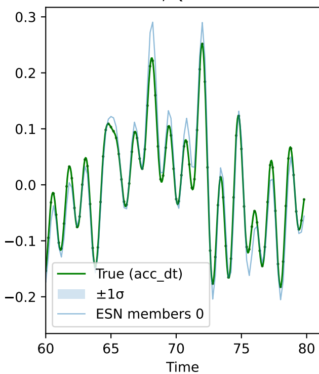
N=5, Qubit=3
