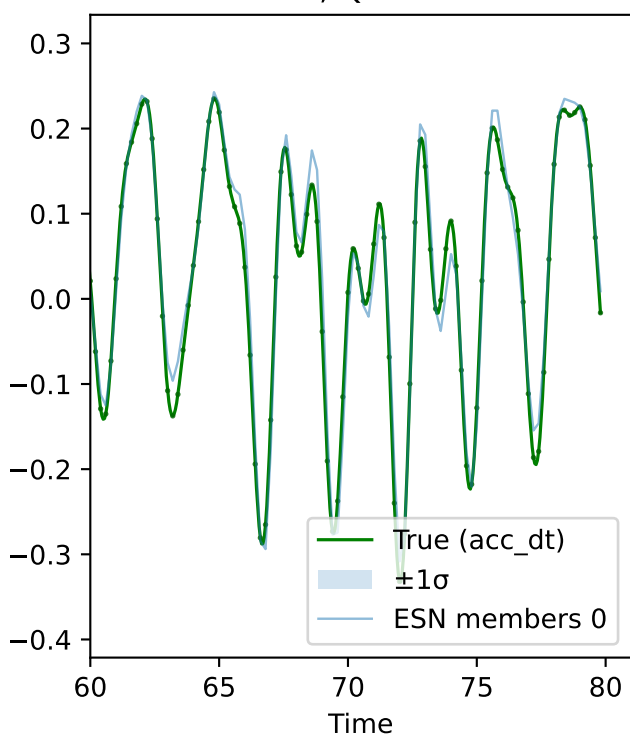
N=5, Qubit=3
